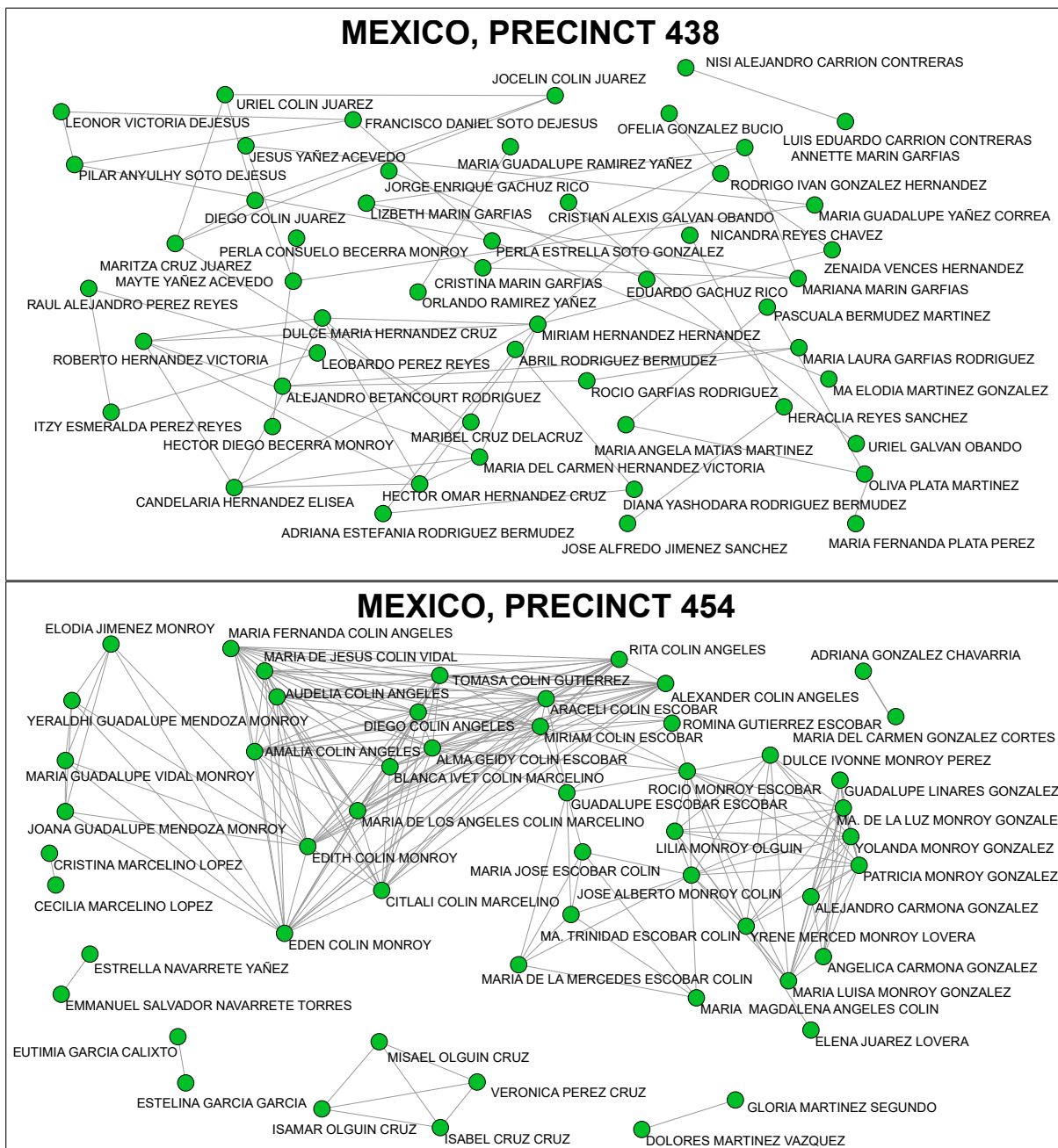
Figure A2: Two networks with individual names as nodes. Top panel: México, precinct 438 (Number of nodes=52, Largest Eigenvalue = 5.08). Bottom panel: México, precinct 454 (Number of nodes=53, Largest Eigenvalue = 15.22)
